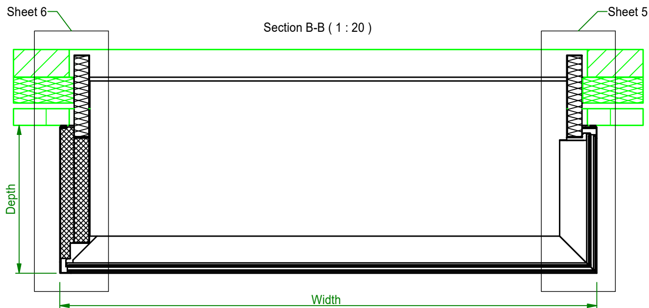
Wall and opening dimensions: Sheet 2
