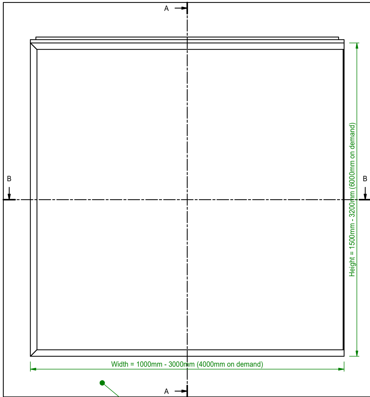
Wall and opening dimensions: Sheet 2
